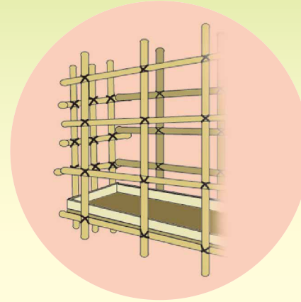
Double row scaffold and working platform
