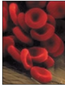
Inhibition of certain enzymes in red blood cells
